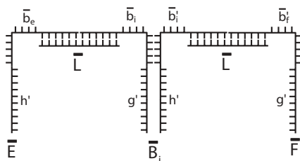
Fig. 2. A trimer consisting of the units \bar{E} , \bar{B}_i , and \bar{F} linked together by the strand \bar{L} . The single-stranded regions \bar{b}_e , \bar{b}_i , \bar{b}'_i , and \bar{b}_f serve as recognition sites for the template-directed construction of the complementary trimer
