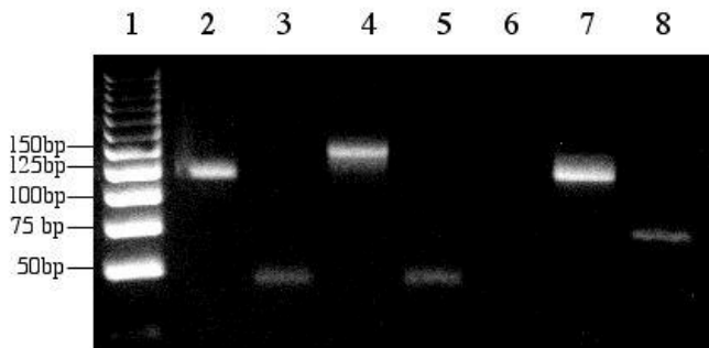
Fig. 7. Electrophoresis results. Lane 1: molecular size marker ladder (25 bp). Lane 2: amplification of \alpha \dots \gamma strands (120 bp); lane 3: amplification of \gamma \dots \beta strands (45 bp); lane 4: cross pairing amplification of \alpha \dots \gamma and \gamma \dots \beta (150 bp). Lane 5: positive control by PCR( \gamma, \bar{\beta} ), with \gamma at position -45; lane 6: negative control by PCR( \gamma', \bar{\beta} ); lane 7, 8: positive controls by PCR( \gamma_1, \bar{\beta} ) and PCR( \gamma_2, \bar{\beta} ) respectively, with \gamma_1 at position -125 and \gamma_2 at position -75
