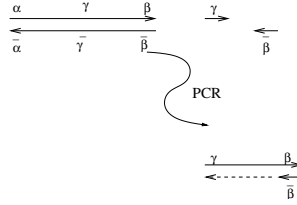
Fig. 4. Second step based on PCR
