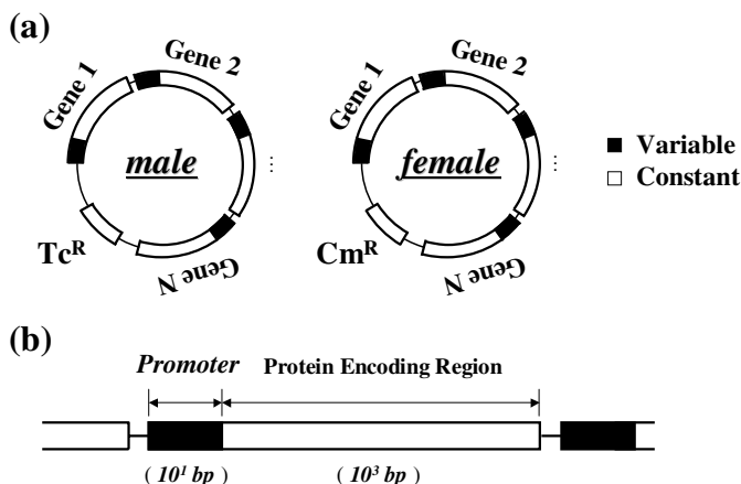
Fig. 2. Configuration of Plasmid DNA Memory
