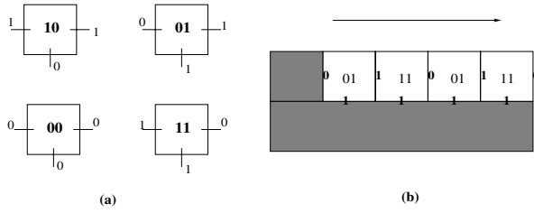
Fig. 1. (a) The parity tile system. (b) Illustrating the action of the parity tile system on the "input" string 1111. The arrow at the top represents the order in which tiles must attach in the absence of errors
