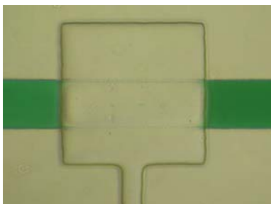
Fig. 6. A fully closed pneumatic valve ( 300 \times 300\text{ }\mu\text{m} square) over a 100\text{ }\mu\text{m} channel, effectively blocking the channel
