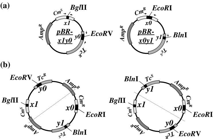
Fig. 4. (a) Plasmids for preliminary experiment. Amp R , Cm R and Tc R indicate antibiotic resistance genes. Cm S and Tc S indicate nonfunctional genes produced by replasing x0 and y0 to x1 and y1 , respectively. Arrows indicate primer annealing sites of PCR. (b) Predicted structures of fusion plasmid. Two possible structures are shown
