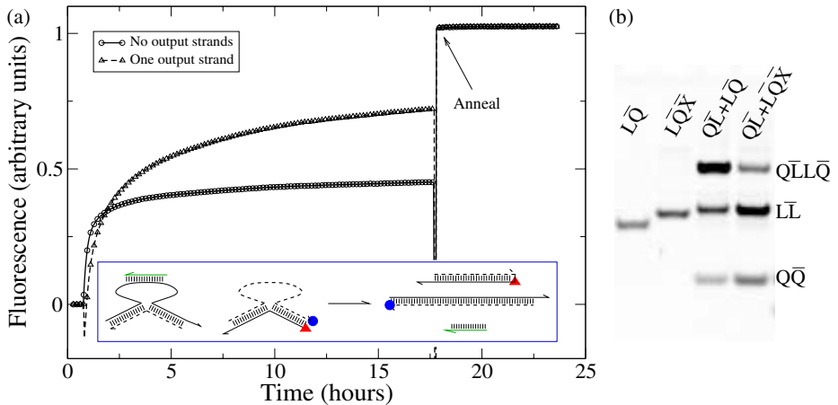
Fig. 8. (a) Comparison of the reactions between the two unmodified loops Q\bar{L} and L\bar{Q} and the reaction between Q\bar{L} and L\bar{Q}\bar{X} . The experiment was performed in TAE buffer (pH 8, 12.5 mM Mg^{++} ) at a temperature T = 20^\circ\text{C} with an initial reactant concentration c = 0.5 \mu M. The locations of the dye label, quencher and output strand \bar{X} are as indicated in the inset. (b) Reactants and reaction products for the reaction between Q\bar{L} and L\bar{Q}\bar{X} . Far left lane: Loop Q\bar{L} . Center left lane: Modified loop L\bar{Q}\bar{X} . Center right lane: Products of the reaction between Q\bar{L} and L\bar{Q} . Far right lane: Products of the reaction between Q\bar{L} and L\bar{Q}\bar{X}
