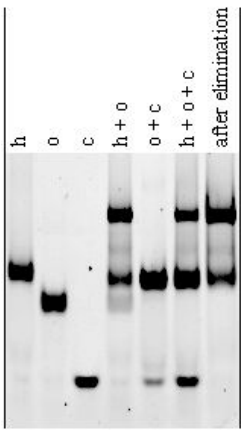
Fig. 7. Experimental results of elimination
