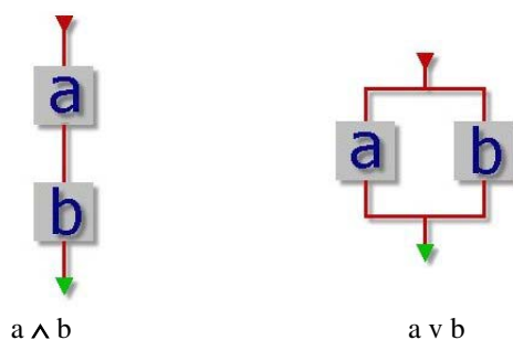
Fig. 1b. AND operations can be made by having two selectors in sequence, while an OR operation is made by two selectors in parallel
