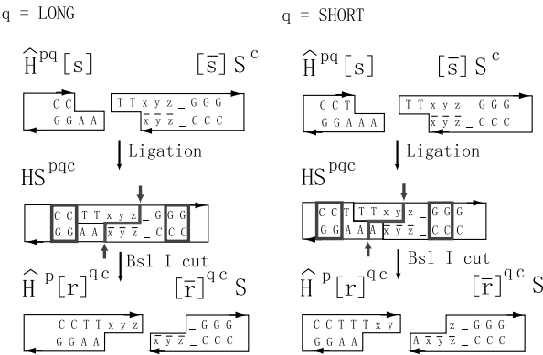
Fig. 3. Step 1 of the operation of ADTM. The current state q and color c are initially encoded in the duplex portion of the Head-Molecule and the Symbol-Molecule, respectively. After the ligation and cleavage, both the sticky ends of the new Head-Molecule and Symbol-Molecule encode the current state q and the current color c . The encoding scheme of c is described in Table 1. Bsl I recognition sites and cleavage sites are indicated with boxes and pairs of bold arrows, respectively
