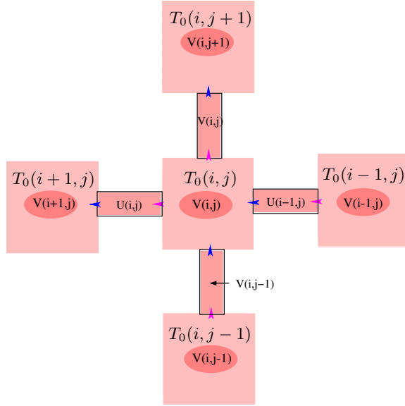
Fig. 1. Tile T_0(i, j) takes input U(i-1, j) and V(i, j-1) ; determines V(i, j) = U(i-1, j) \text{ OP}_1 V(i, j-1) and U(i, j) = U(i-1, j) \text{ OP}_2 V(i, j-1) ; displays V(i, j)
