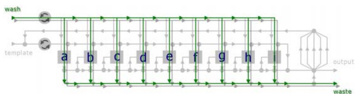
Fig. 5b. The flow pattern for the washing step. Notice that the memory channels are not affected in this step
