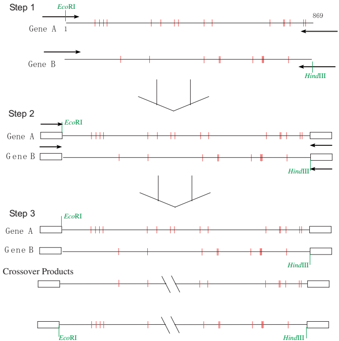
Fig. 3. PCR steps for achieving one-point crossover
