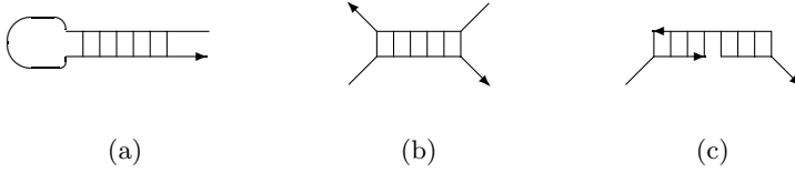
Fig. 1. Types of intramolecular (a) and intermolecular (b), (c) hybridizations
