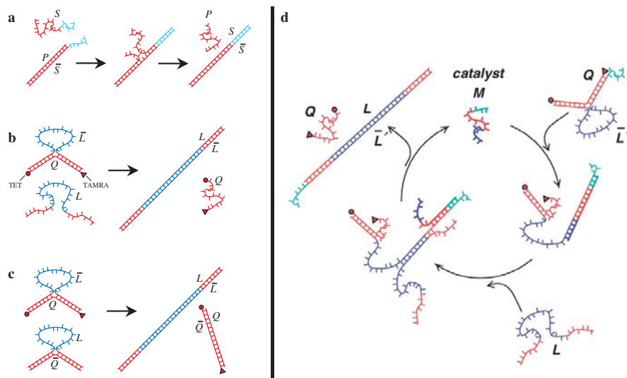
Fig. 1. (a) Single-stranded toehold allows rapid displacement of P by S . (b) The Q\bar{L} + L \rightarrow Q + L\bar{L} reaction is slow. (c) The Q\bar{L} + L\bar{Q} \rightarrow Q\bar{Q} + L\bar{L} reaction is even slower. (d) Strand M catalyzes the Q\bar{L} + L \rightarrow Q + L\bar{L} reaction
