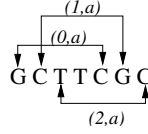
Fig. 3. Coding used to simulate three different states
