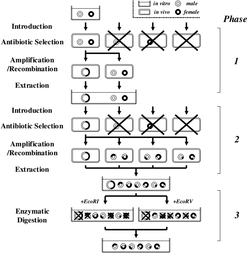
Fig. 3. Procedure of Crossover Operation
