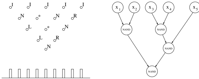
Fig. 1. An example of a template and the Boolean formula it encodes [10]. Under the template of labeled pawns one can see its vertical section. In this example four N -tiles are used for computation while ten tiles are needed in total (besides the input)
