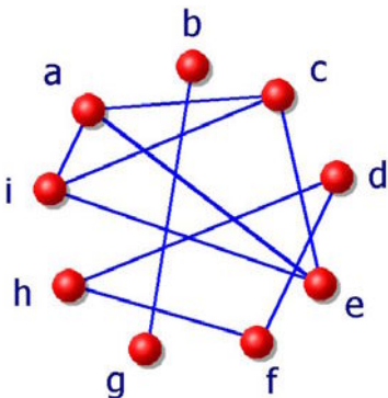
Fig. 4. An N=9 instance of the clique problem. The maximum clique is given by ACEI, represented by 101010001
