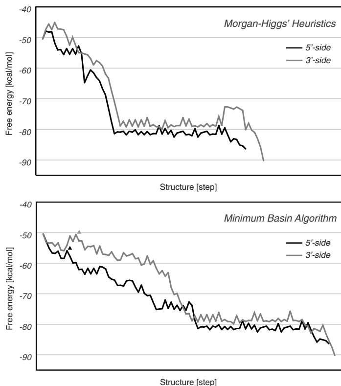
Fig. 5. Free Energies along the Structural Transition Path. These are the paths from the mfe structure when the hairpin does not hybridize with any input DNA to the mfe structure when the hairpin hybridizes with one of the input DNA. The vertical axis is the free energy of the structure given on the horizontal axis. The “addition” or “removal” of a base pair is one step involved in changing the secondary structure along the horizontal axis. In the lower graph, the lower left corner of the triangle shows the structure that is thought to be a kind of barrier
