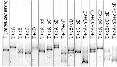
Fig. 5. Experimental results of distinguishing of all 16 states
