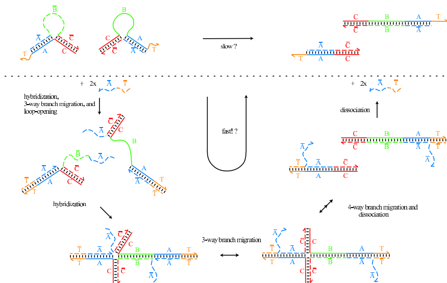
Fig. 2. Two copies of strand M catalyze the Q\bar{L} + L\bar{Q} \rightarrow Q\bar{Q} + L\bar{L} reaction of Fig. 1c. Here, subsequences of each strand are explicitly labeled, and the necessary toeholds are added. Thus, M = \bar{T}\bar{A} , Q = CAT , \bar{L} = \bar{A}\bar{B}\bar{C} , \bar{Q} = \bar{A}\bar{C} , and L = CBAT . The dotted line separates uncatalyzed reactions from those that occur only in the presence of catalyst strand \bar{T}\bar{A}
